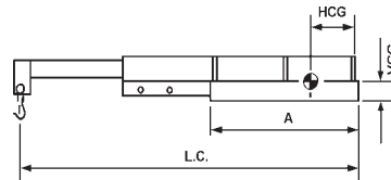
T24H Series Hydraulic Telescopic Boom
